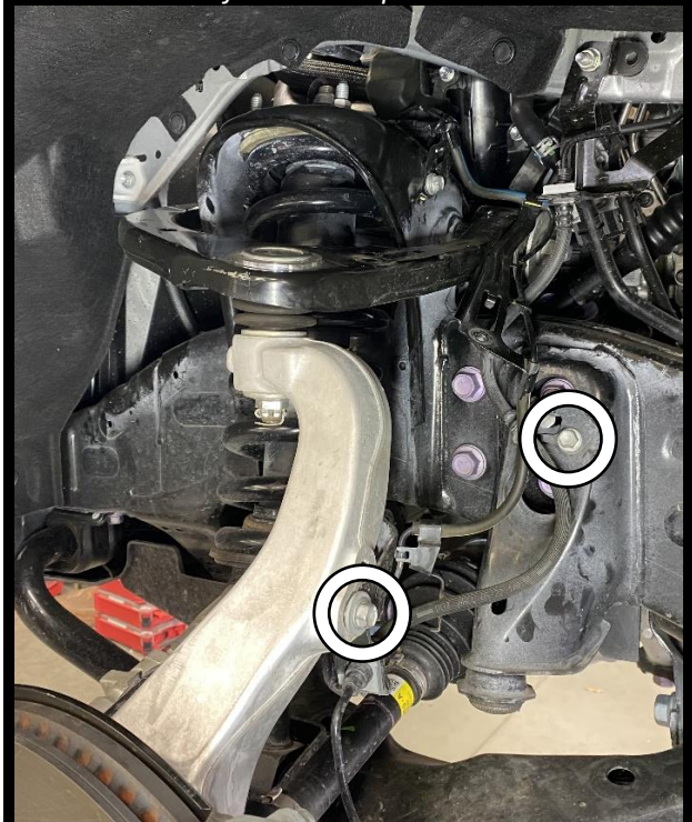
Figure 7: Remove ABS and brake brackets from frame and spindle.
